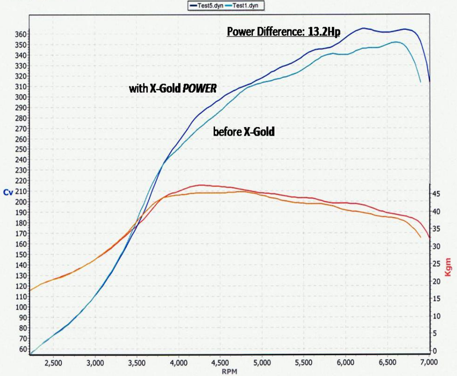
Torque/Engine Power
